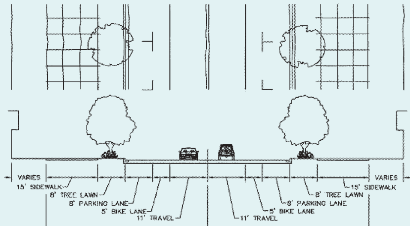
RECOMMENDED MIXED-USE STREET SECTION
