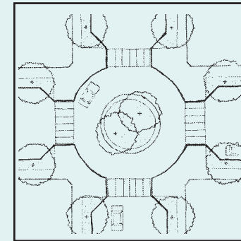
TRAFFIC CIRCLE WITH INTERSECTION BULB-OUTS
