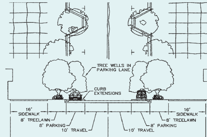
RECOMMENDED MAIN STREET SECTION
