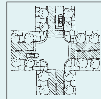
RAISED CROSSWALK
